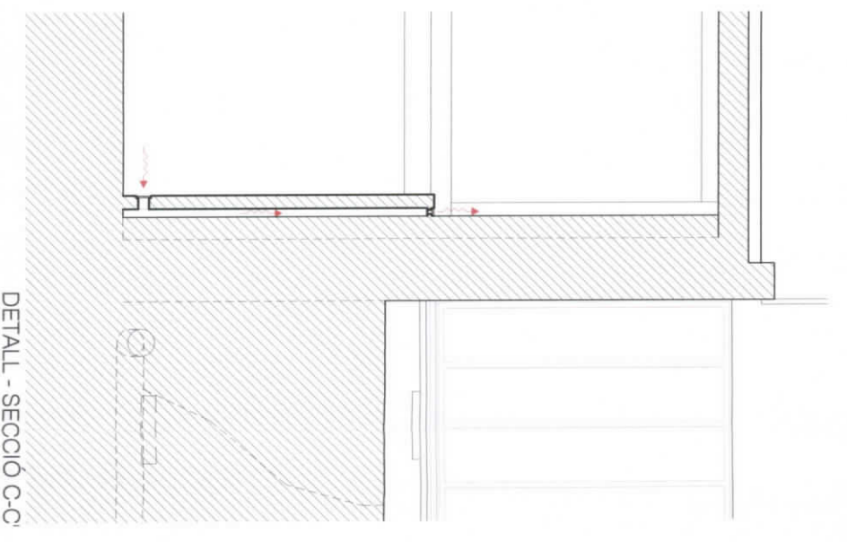
REIXA LINEAL SENSE BASTIDOR 500x100mm.
